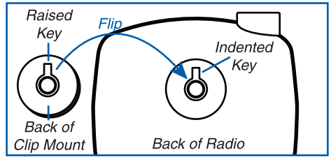
Fig. 1: Attach Clip Mount
